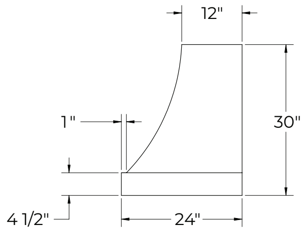
48" SIDE VIEW
