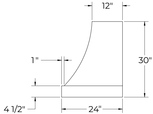
36" SIDE VIEW
